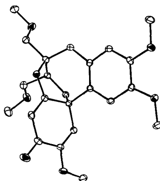
Figure 1. X-ray structure of 26
